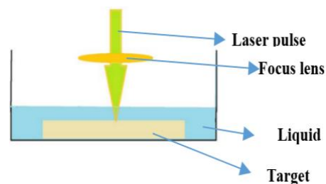
Fig. 1. The experimental arrangement for producing Ag NPs by laser ablation.
