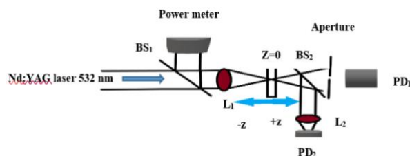
Fig. 2. Arrangement of Z-scan method.
