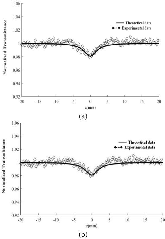
Fig. 9. Opened aperture Z-scan experimental data (dashed-diamond line) and theoretical curve (solid line) calculated using Eq. 4 for Ag NPs at the optimum number of the laser pulses at 900 with two optimum laser energy densities: (a) 0.09\text{J}/\text{cm}^2 and (b) 0.11\text{J}/\text{cm}^2 .
