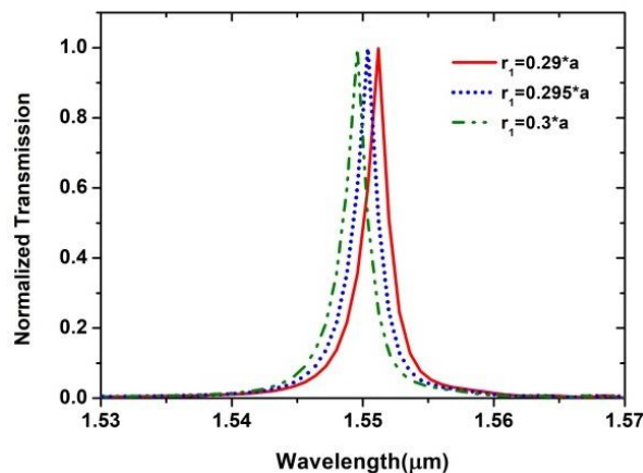
Fig. 7. Normalized transmission spectrum at forward dropping port C for varying radius ( r_1 ) of coupling holes.
