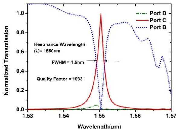
Fig. 3. Normalized transmission at different ports of proposed ADF.
